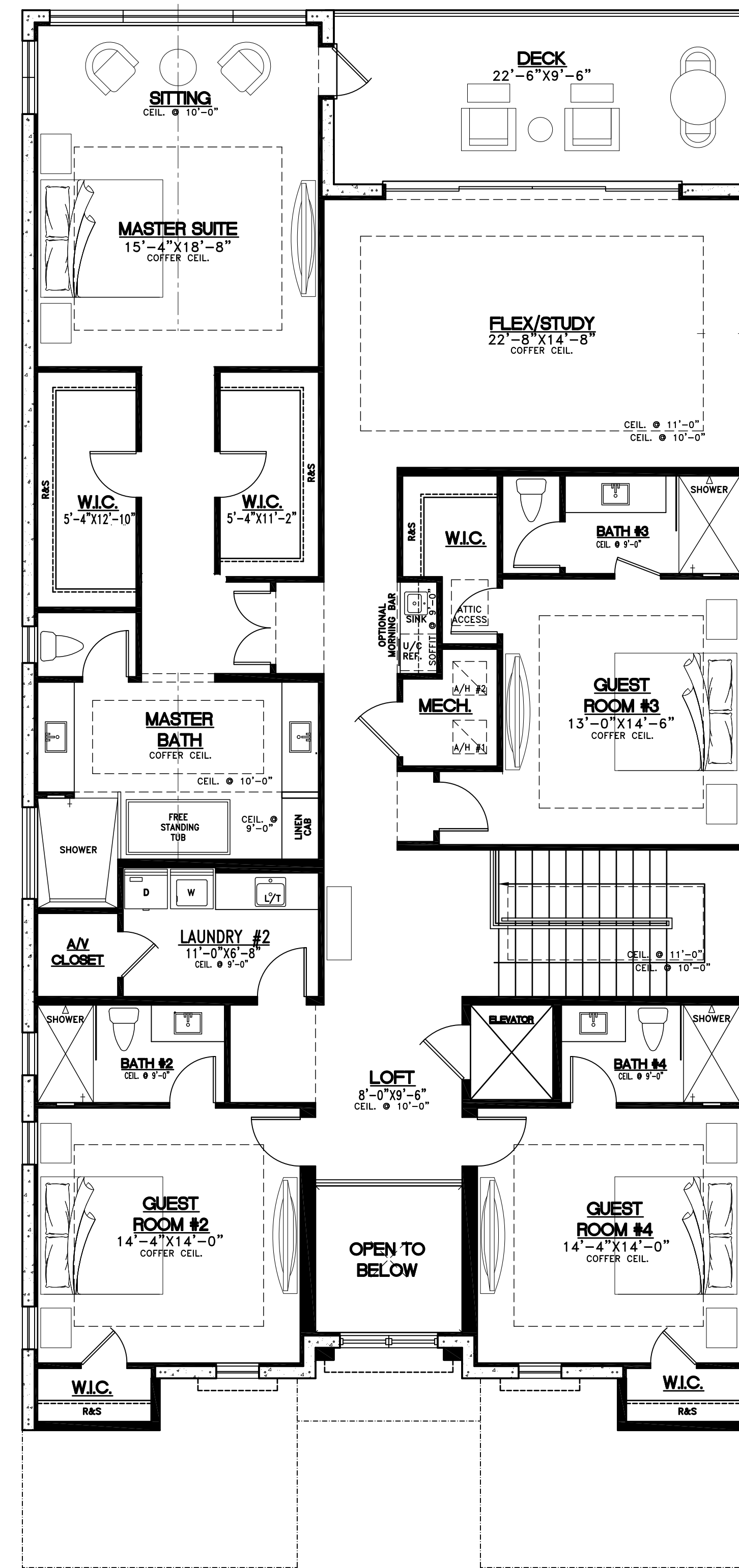
SECOND FLOOR
